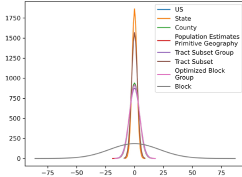
DHC 8-25-2022 Comparison of \mathcal{N}_z(0, \sigma^2) Distributions zCDP Mechanism-Units DETAILED
