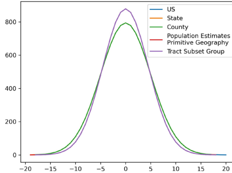
DHC 8-25-2022 Comparison of \mathcal{N}_z(0, \sigma^2) Distributions zCDP Mechanism-Units MULTIG * HISP * HHTENSHORT_2LEV
