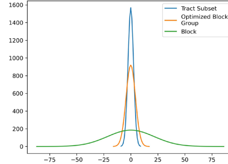
DHC 8-25-2022 Comparison of \mathcal{N}_z(0, \sigma^2) Distributions zCDP Mechanism-Units SEX * HISP * HHTENSHORT_3LEV * RACE * HHAGE * FAMILY_NONFAMILY_SIZE
