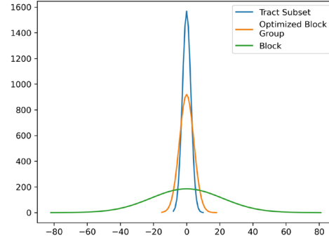
DHC 8-25-2022 Comparison of \mathcal{N}_z(0, \sigma^2) Distributions zCDP Mechanism-Units SEX * HISP * HHTENSHORT_3LEV * RACE * FAMILY_NONFAMILY_SIZE
