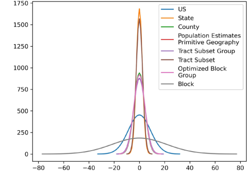
DHC 8-25-2022 Comparison of \mathcal{N}_z(0, \sigma^2) Distributions zCDP Mechanism-Units TENVACGQ
