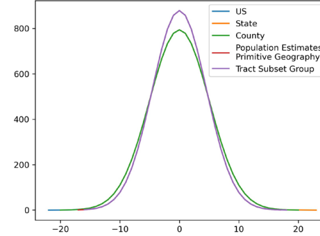
DHC 8-25-2022 Comparison of \mathcal{N}_z(0, \sigma^2) Distributions zCDP Mechanism-Units PARTNER_TYPE_OWN_CHILD_STATUS * SEX * HHTENSHOT_2LEV
