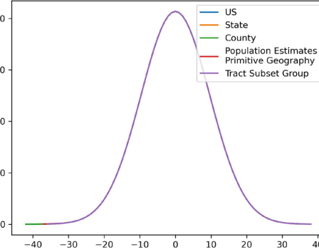
DHC 8-25-2022 Comparison of \mathcal{N}_z(0, \sigma^2) Distributions zCDP Mechanism-Units HISP * HHTENSHORT_2LEV
